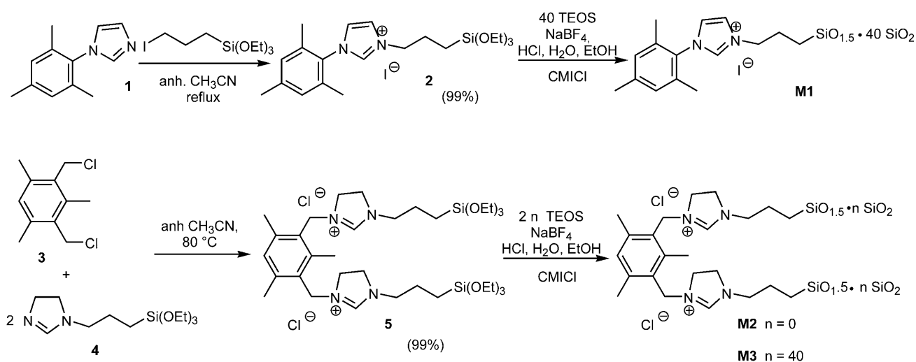
Scheme 1. Synthesis of hybrid silica materials M1–M3 .
