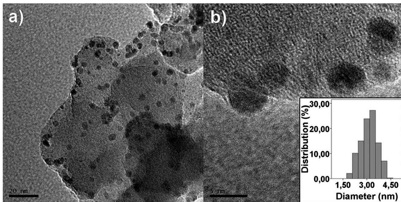
Figure 2. a) and b) HR-TEM micrographs of Pd nanoparticles. The inset in b) shows the particle size distribution (385 particles; mean particle size: 3.1 ± 0.5).
