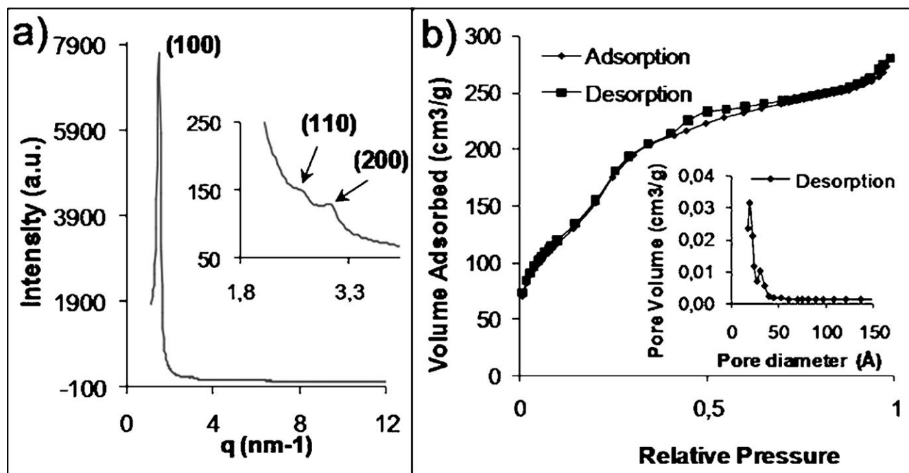
Figure 1. a) p -XRD of M1 ; b) N 2 sorption isotherm of M1 and plot of the pore size distribution.
